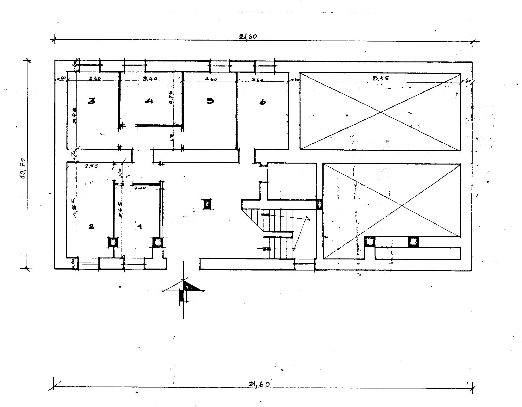
PIANO TERRA
