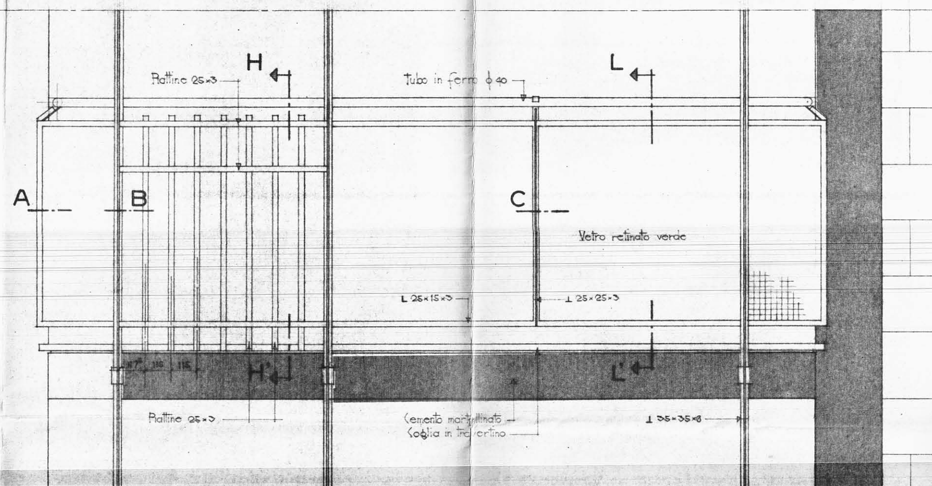
Tubo in ferro Ø 40 Plattine 25x25 1050 765 200 300 80 130-30-3 85
