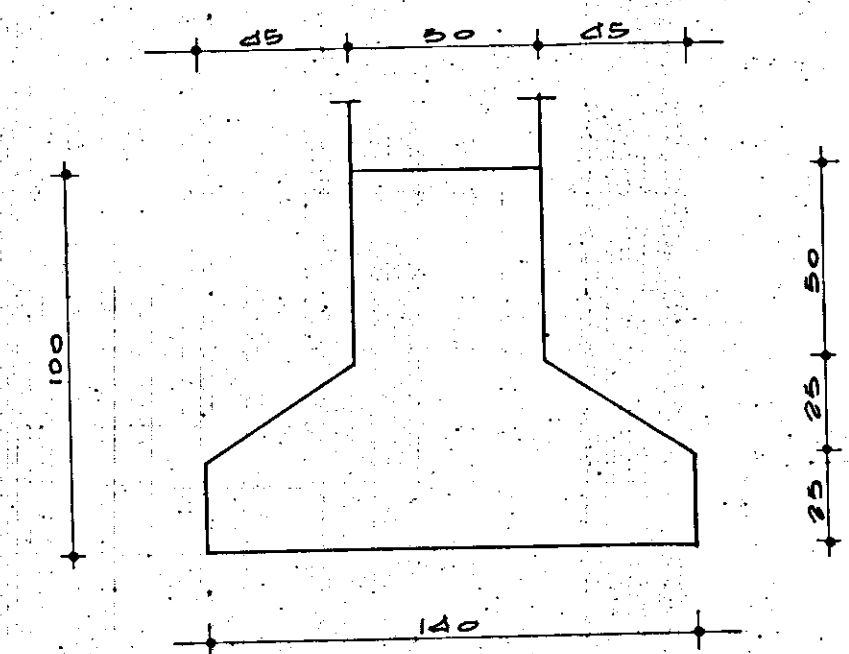
TRAVE 5-6-7-8-10-10'-8'-7'-6'-5'; 12-13-14-15-16-15'-14'-13'-12'
