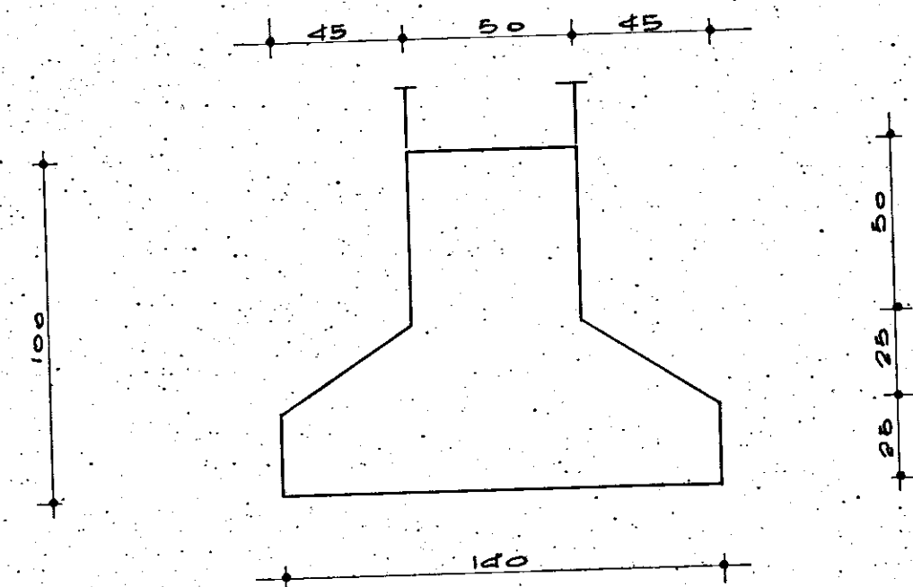
TRAVE 1-2-3-4-4'-3'-2'-1'
