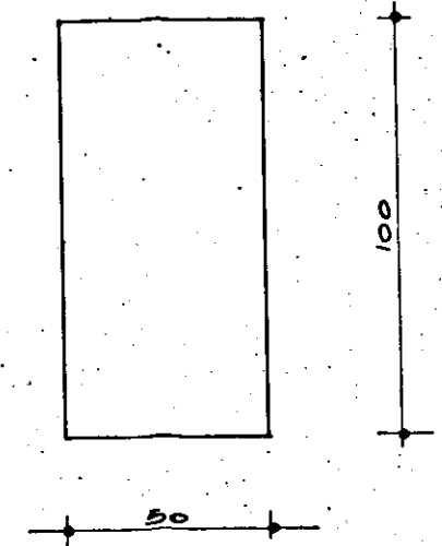
CORDOLI 1-5-12; 1'-5'-12'; 4-9(8-10); 4'-9'(8'-10'); 10-11(15-16); 10'-11'(15'-16);
