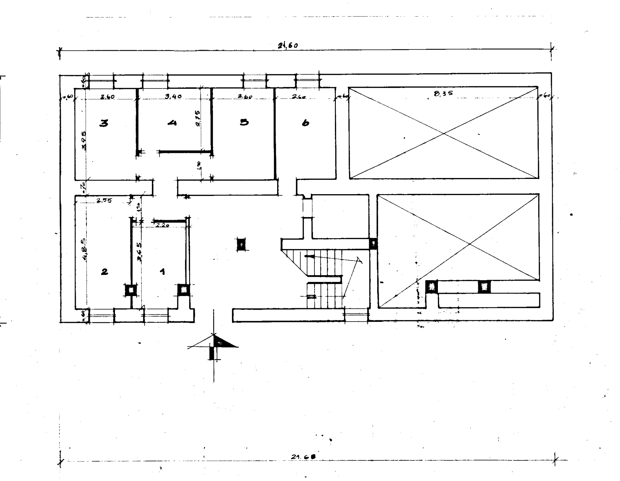
PIANO TERRA
