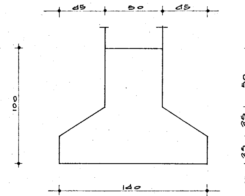
TRAVE 5-6-7-8-10-10'-8'-7'-6'-5'; 12-13-14-15-16-15-14'-13'-12'
