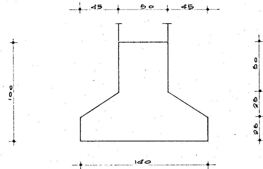
TRAVE 1-2-3-4-4'-3'-2'-1'
