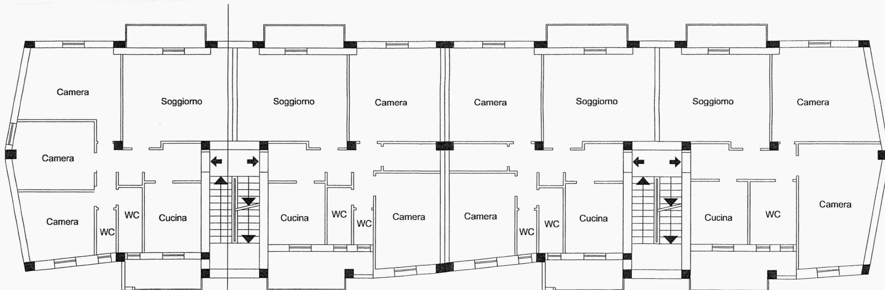
Pianta piano 1-2-3
