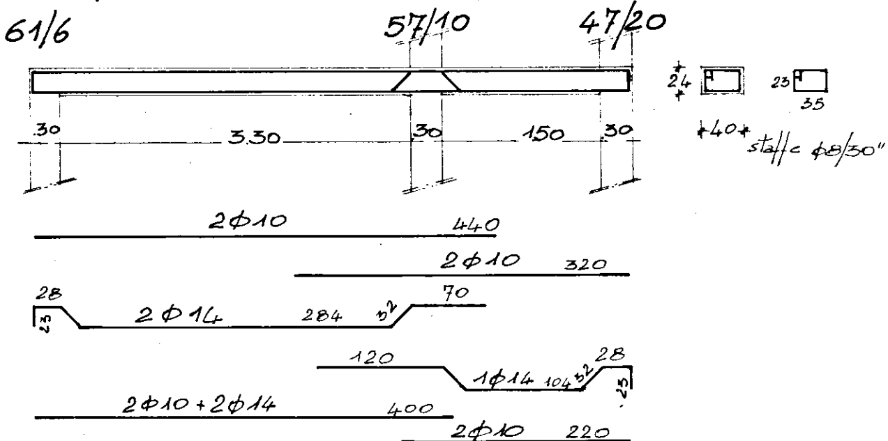
TRAVE 61-57-47; 6-10-20
