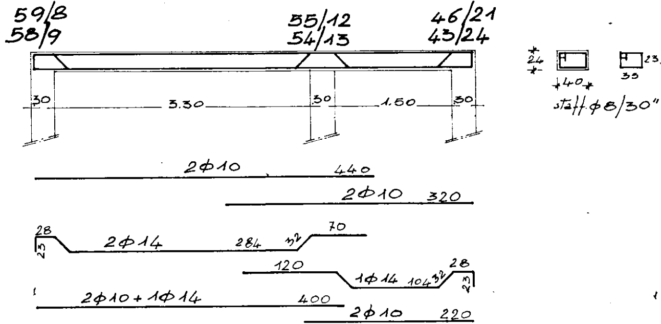
TRAVE 58-54-43; 59-55-46; 9-13-24; 8-12-21
