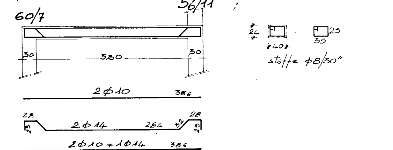
TRAVE 60-36; 7-11
