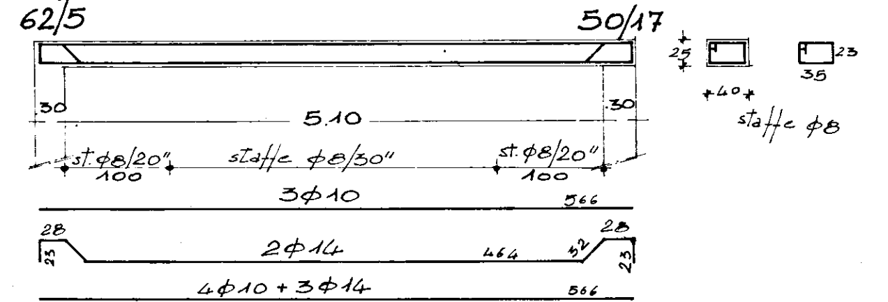
TRAVE 62-50; 5-17
