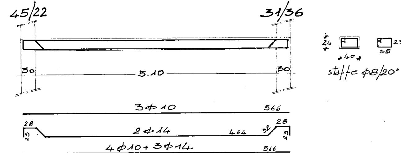
TRAVE 45-31; 22-36
