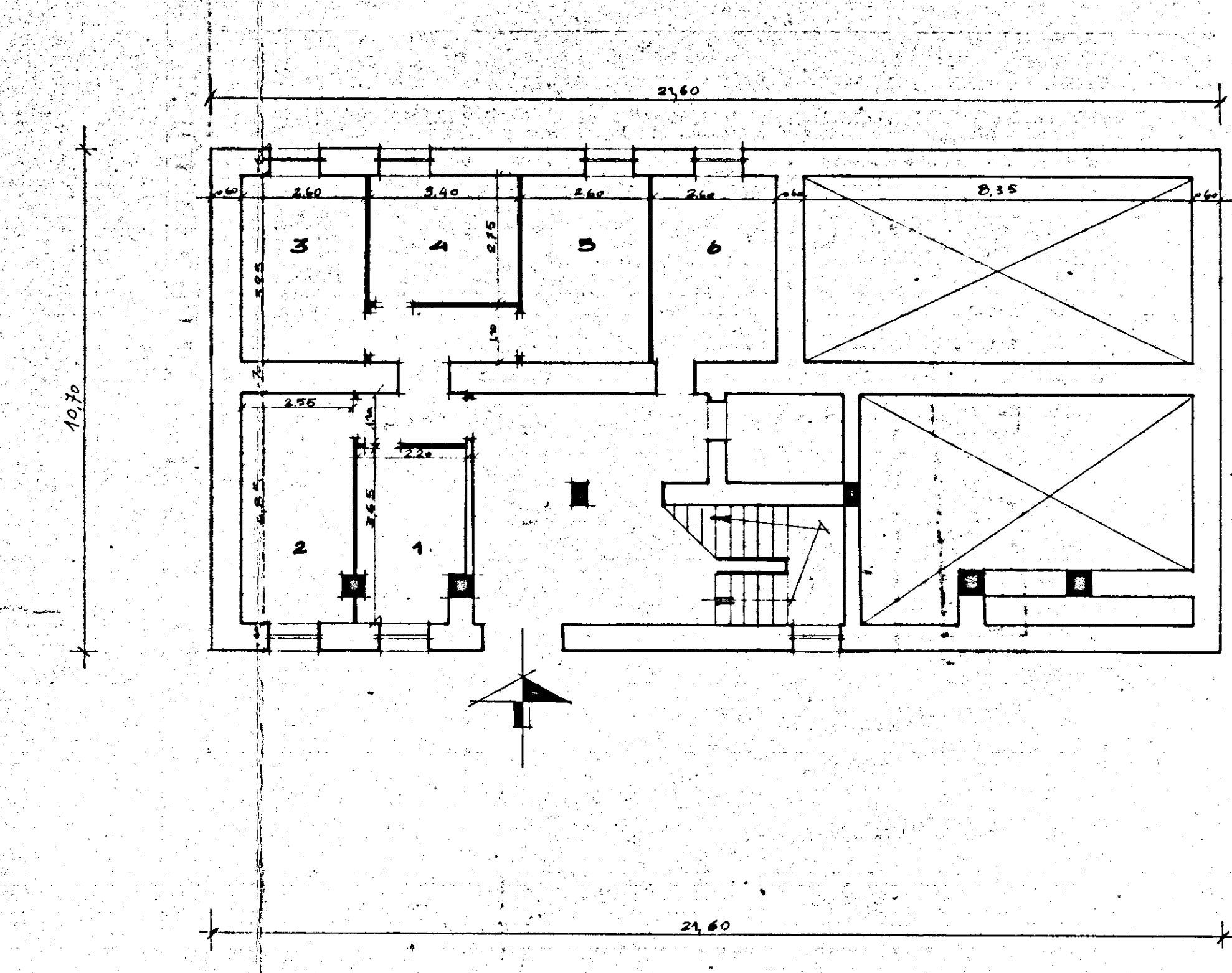
PIANO TERRA
