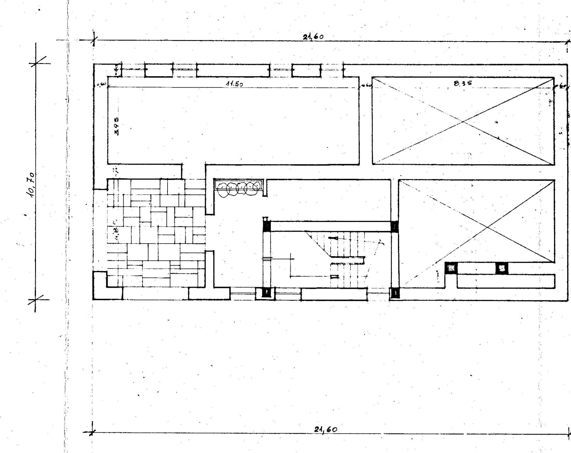
PIANO TERRA
