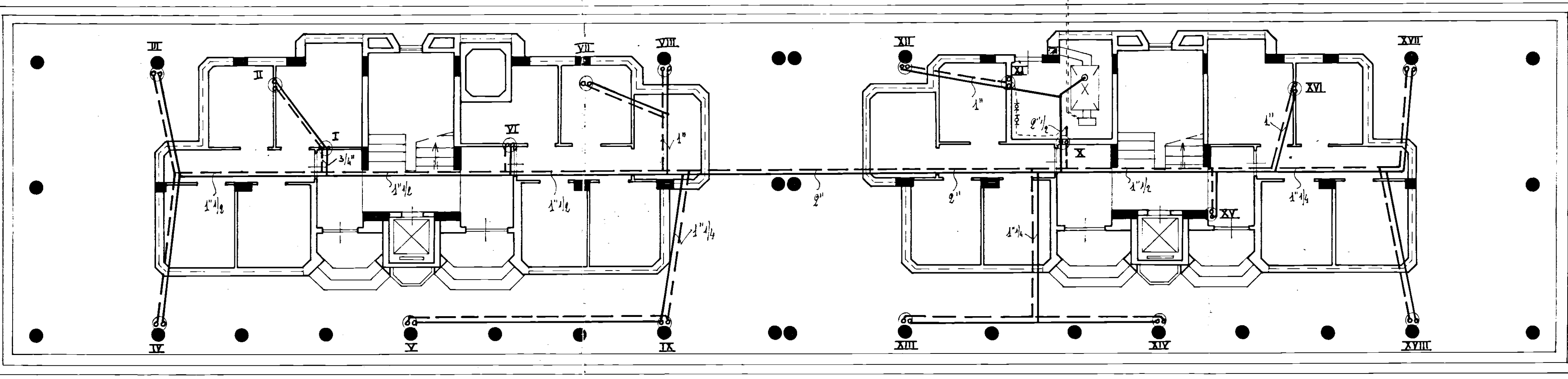
PIANO TERRA
