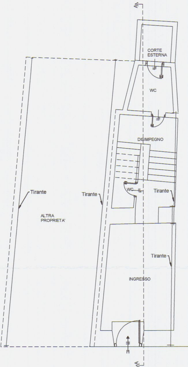
PIANO TERRA
