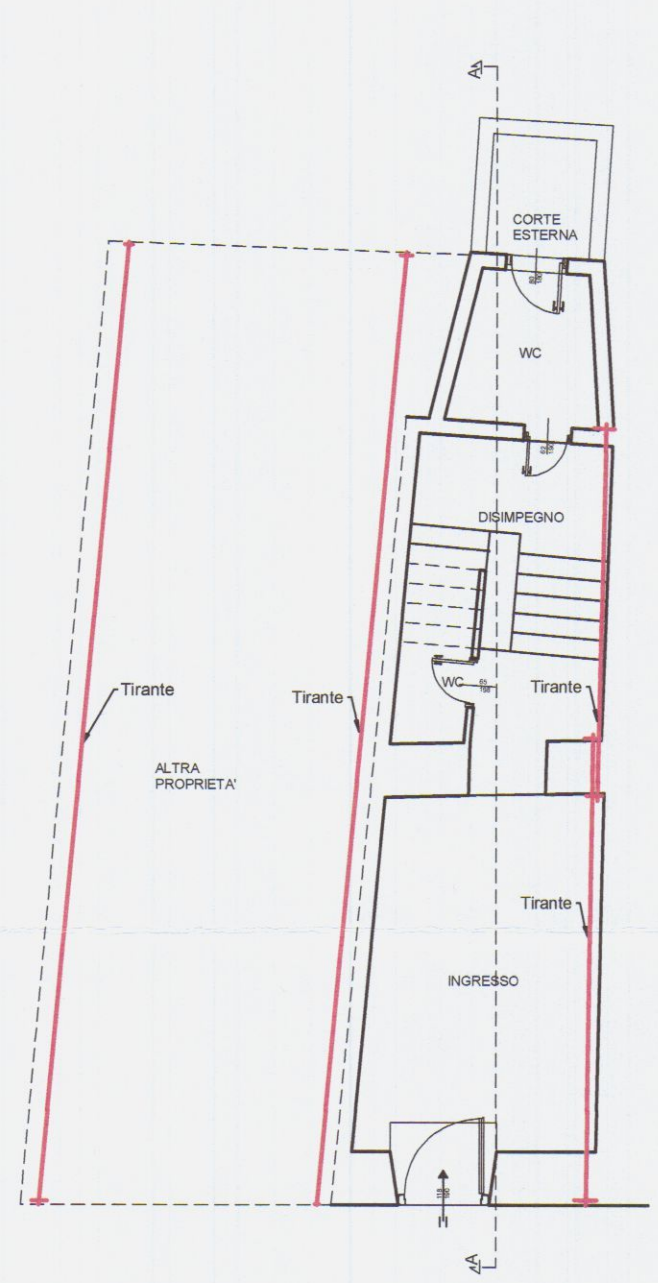
PIANO TERRA
