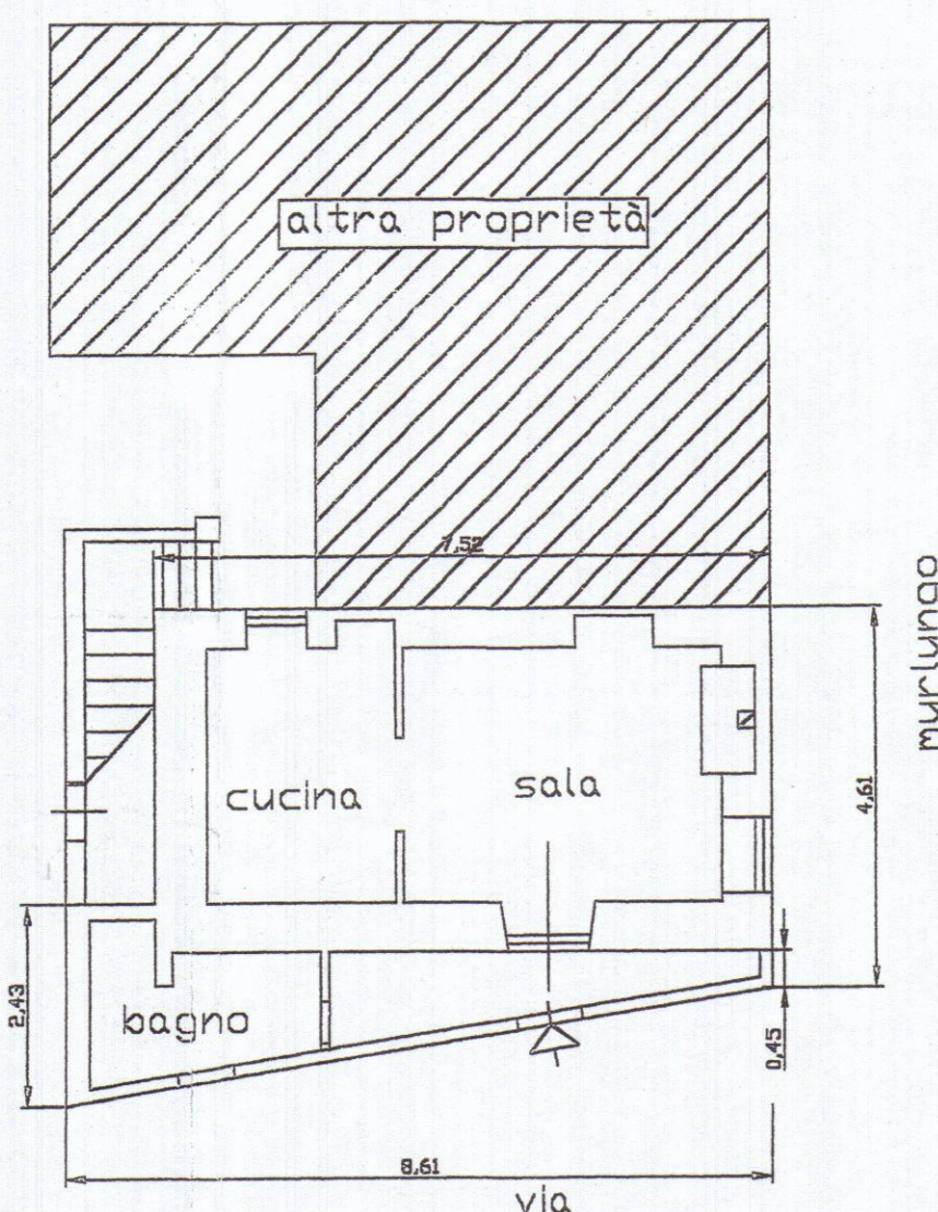
PIANO TERRA
