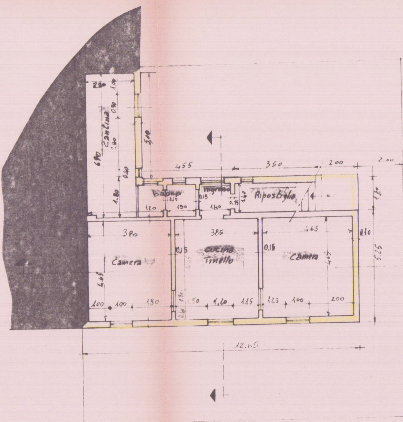
PIANO TERRA
