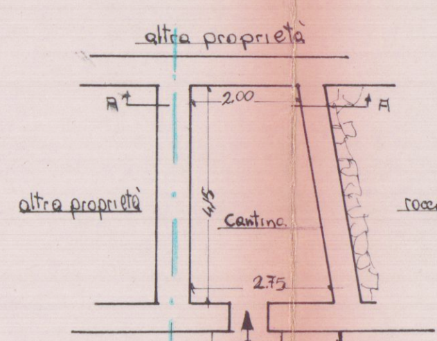
Piano s.i.
