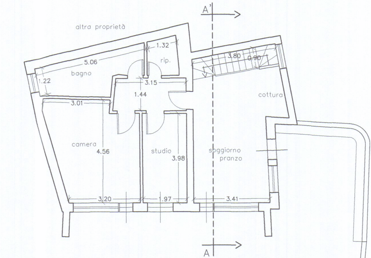
PIANO TERRA
