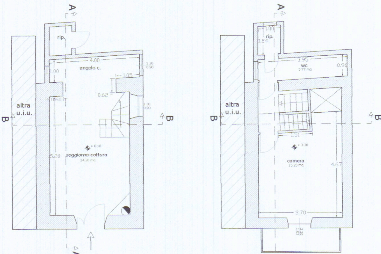
Piano Terra
