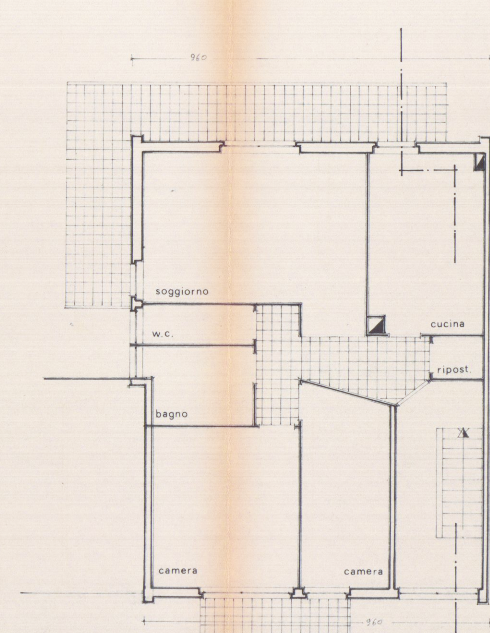
3° PIANO
