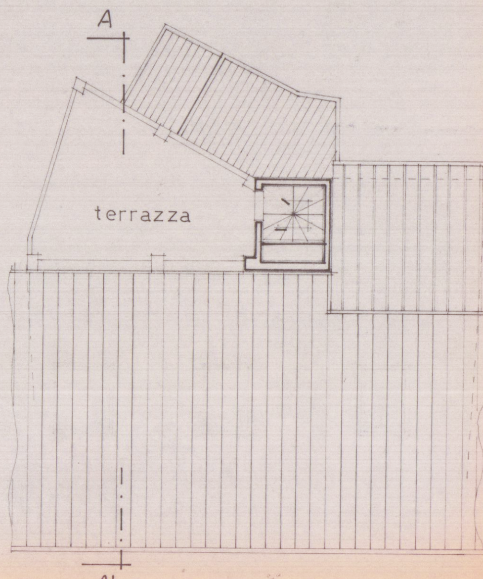
piano quarto
