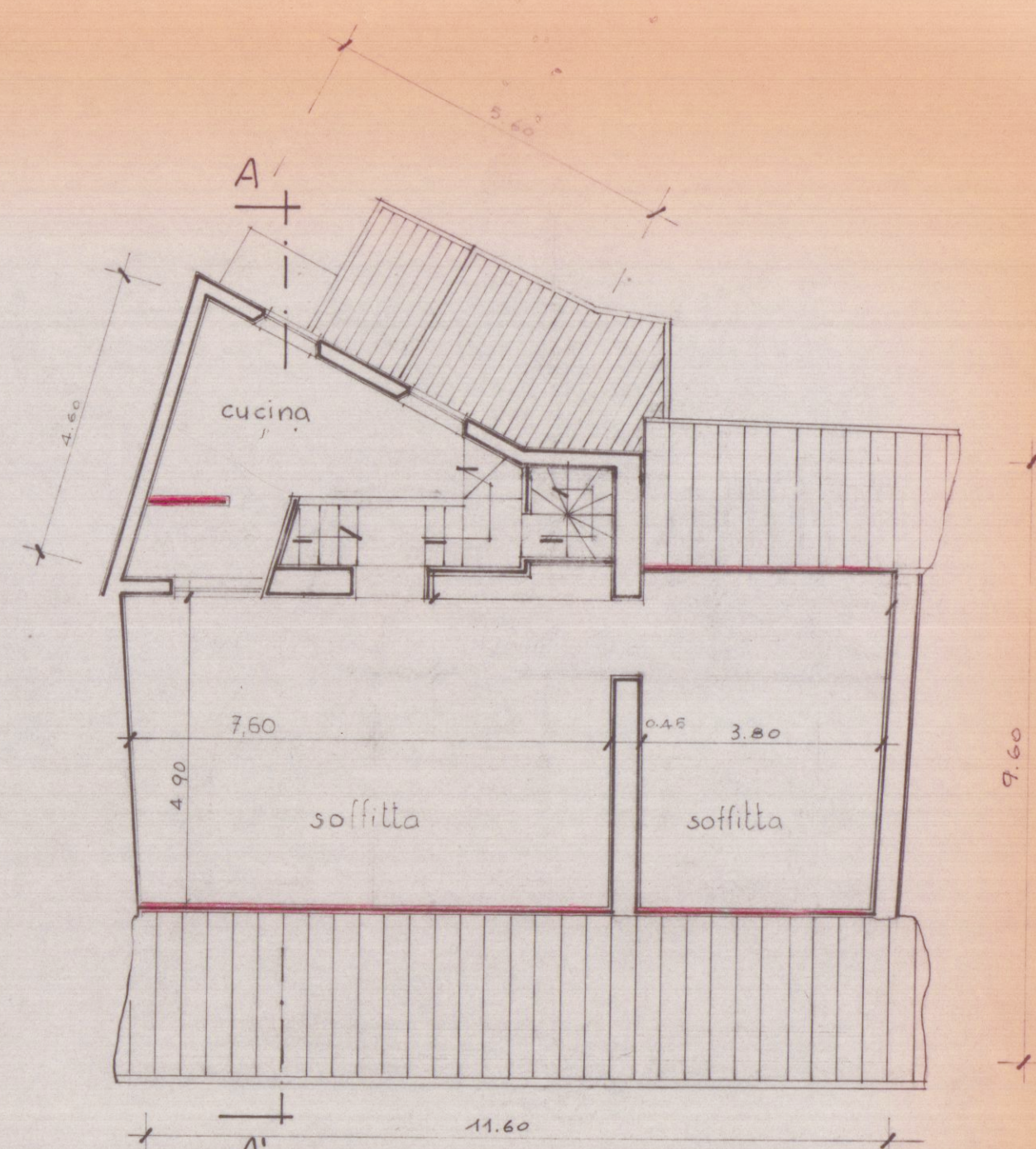
piano quarto
