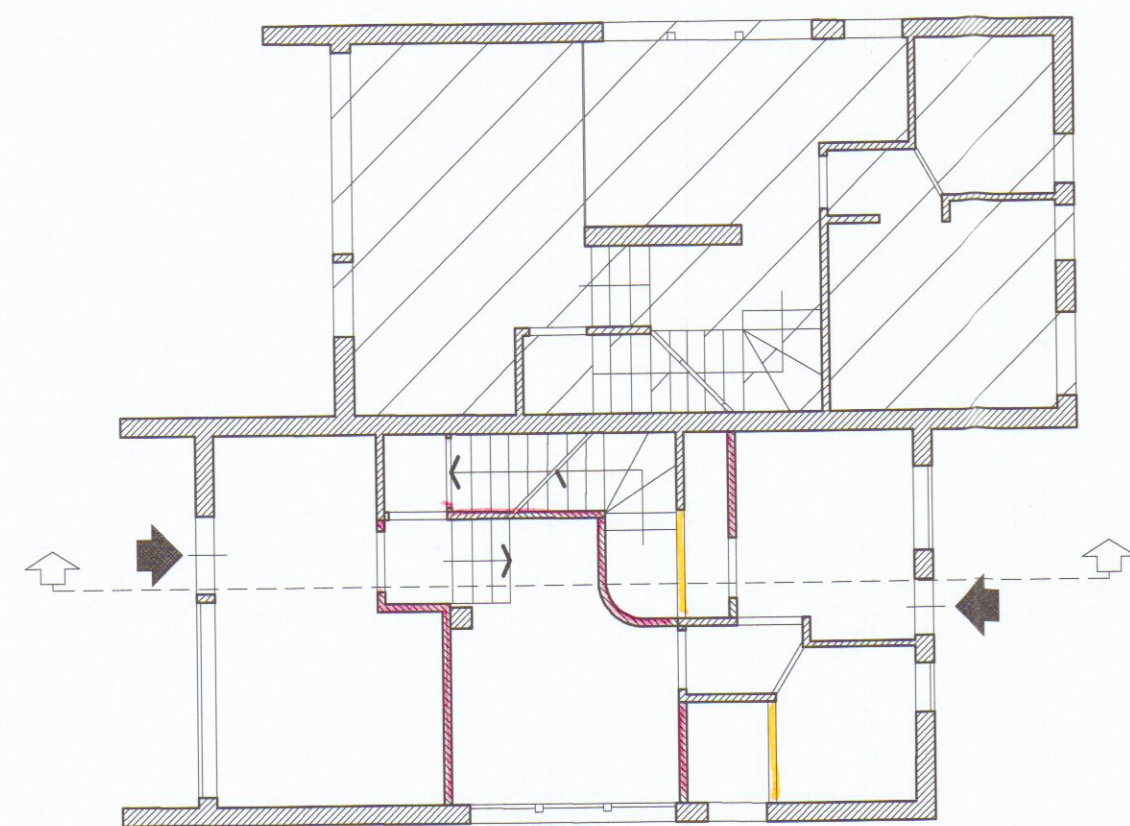
PIANO TERRA
