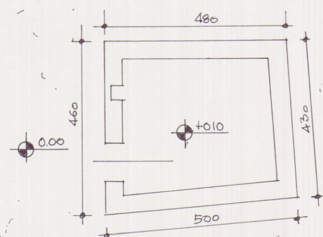
PIANO TERRA
