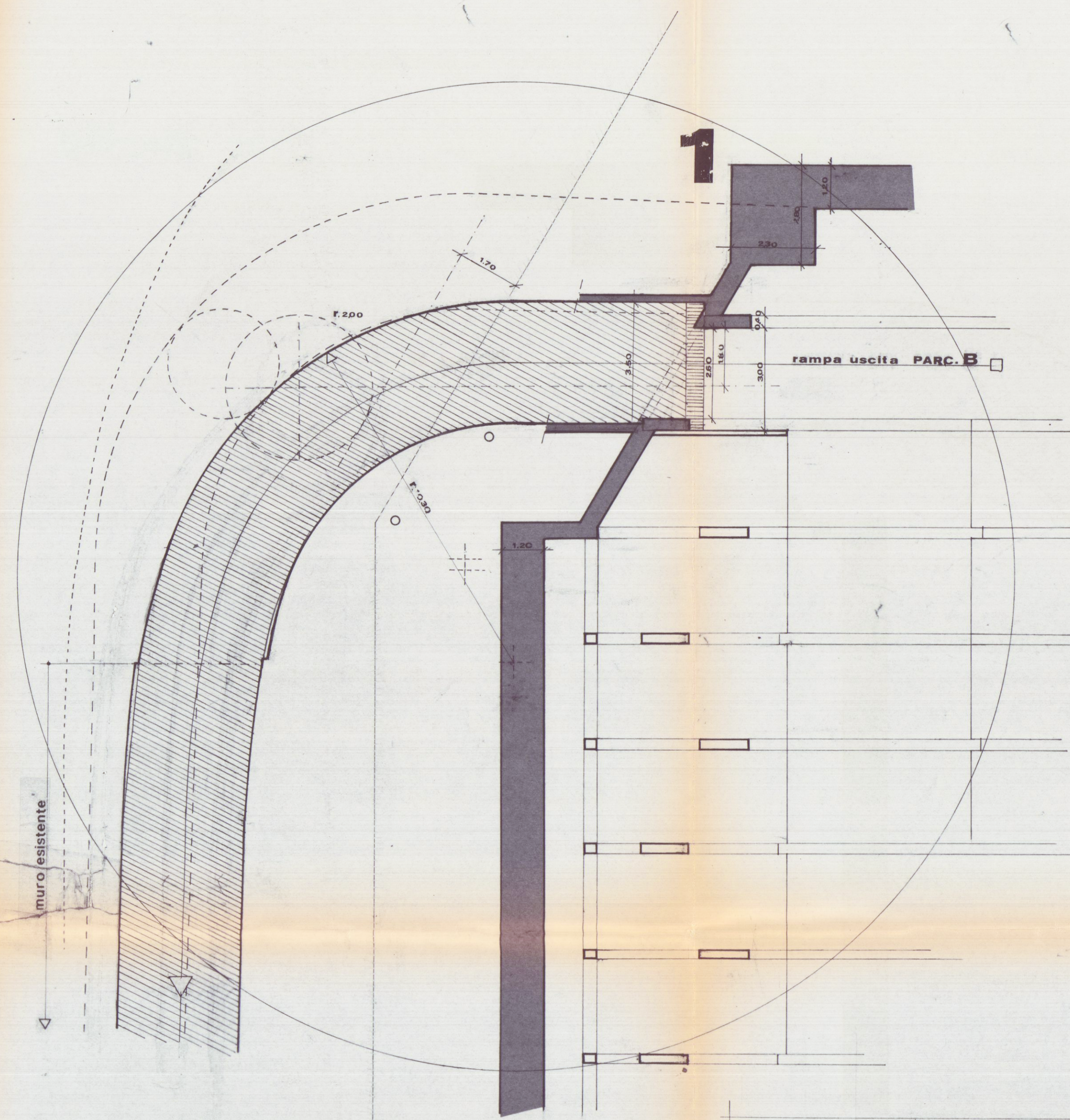
PIANO INTERRATO
