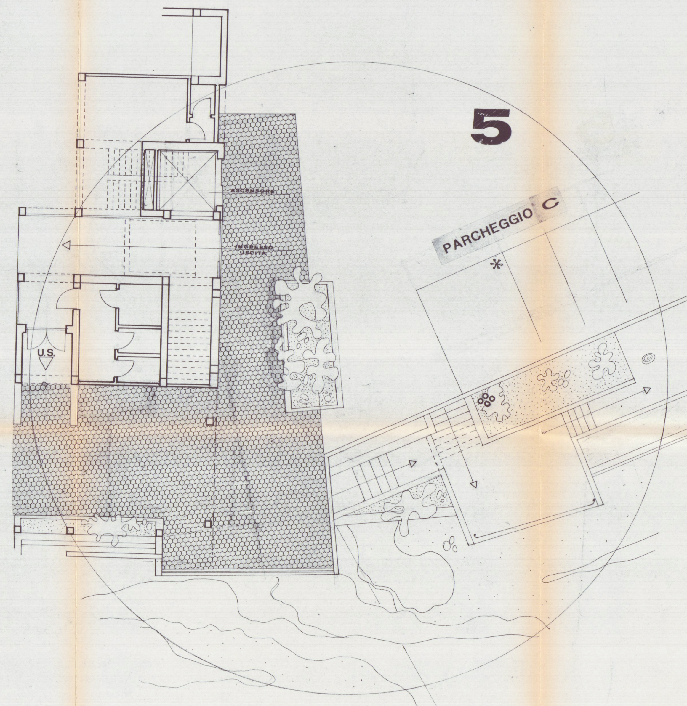
PIANO TERRA
