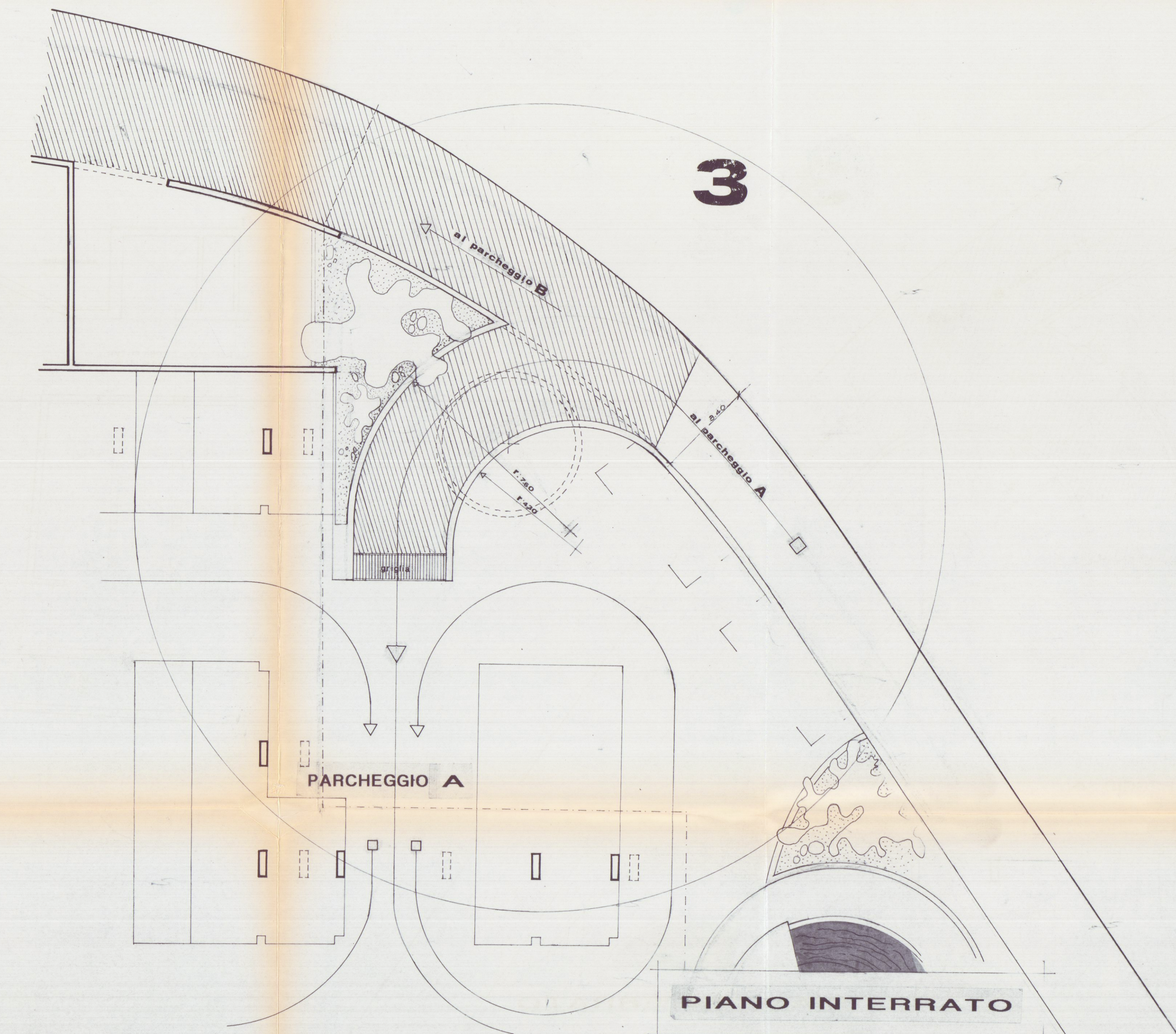
PIANO INTERRATO
