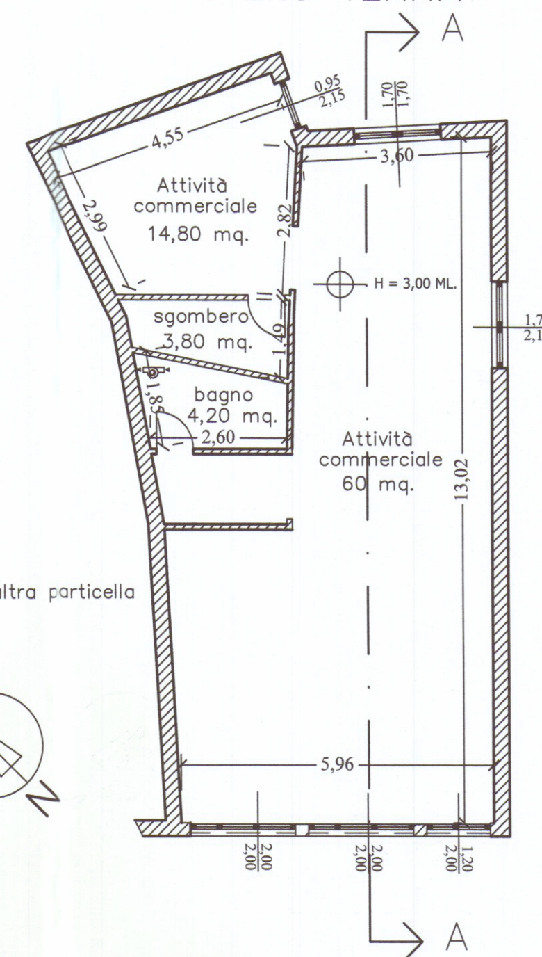
Piano TERRA
