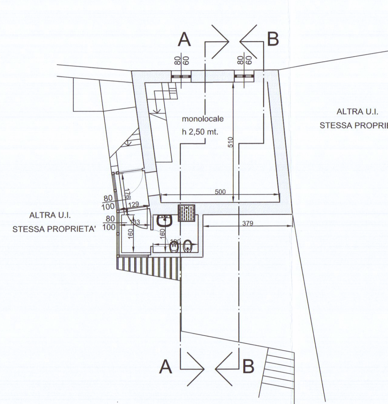
PIANO PRIMC
