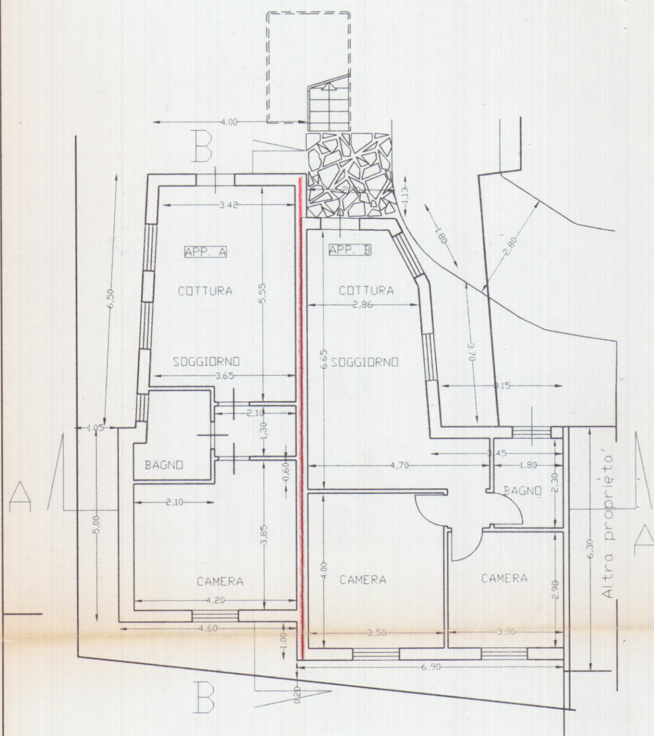
PIANO TERRA
