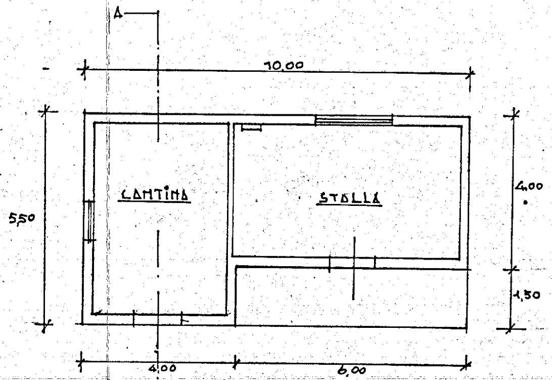
PIANO TERRENO
