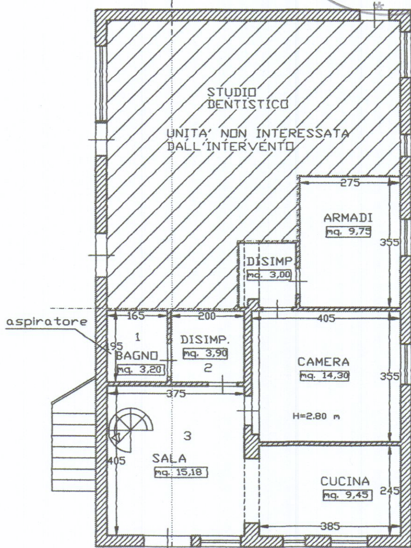
PIANO TERRA
