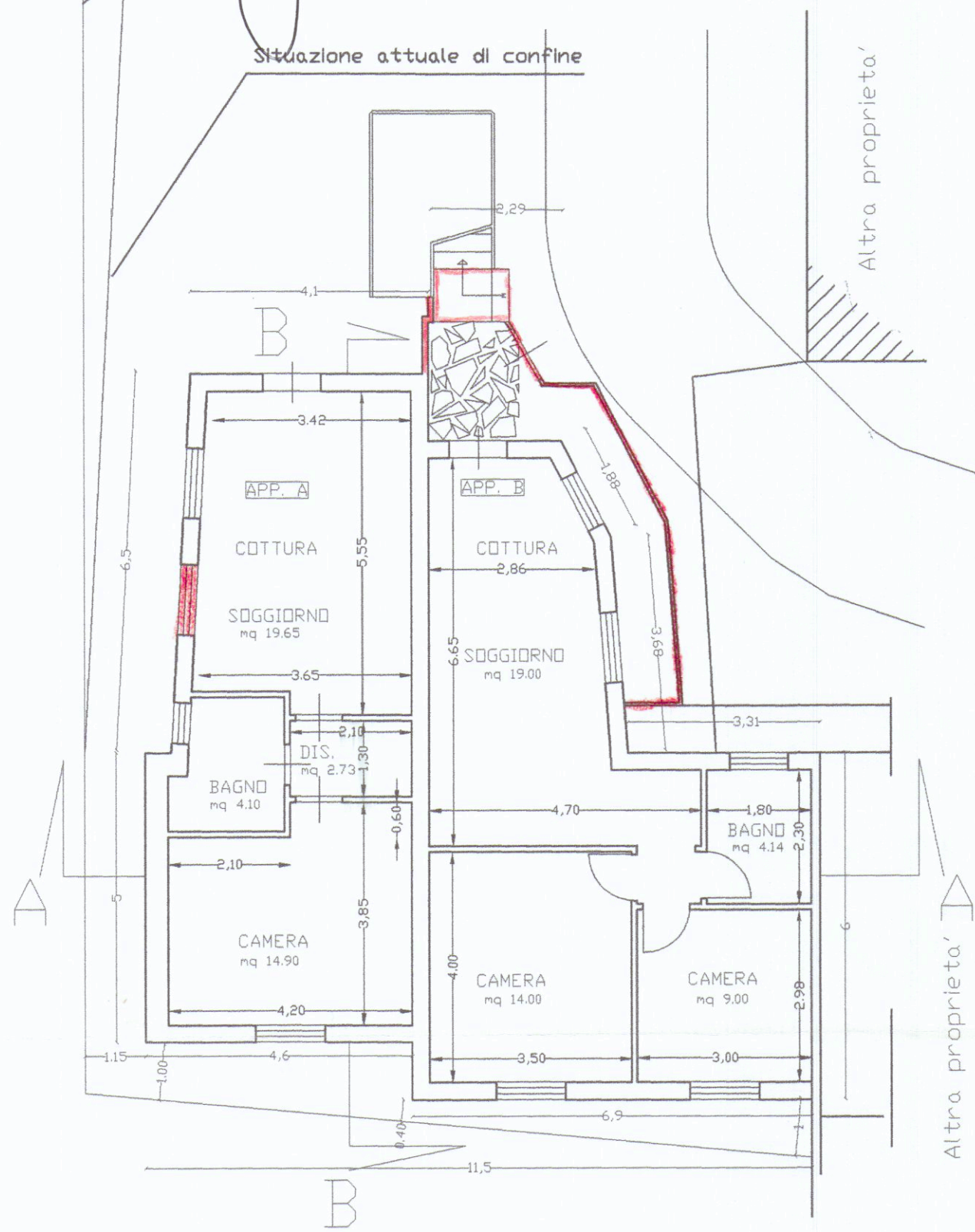
PIANO TERRA
