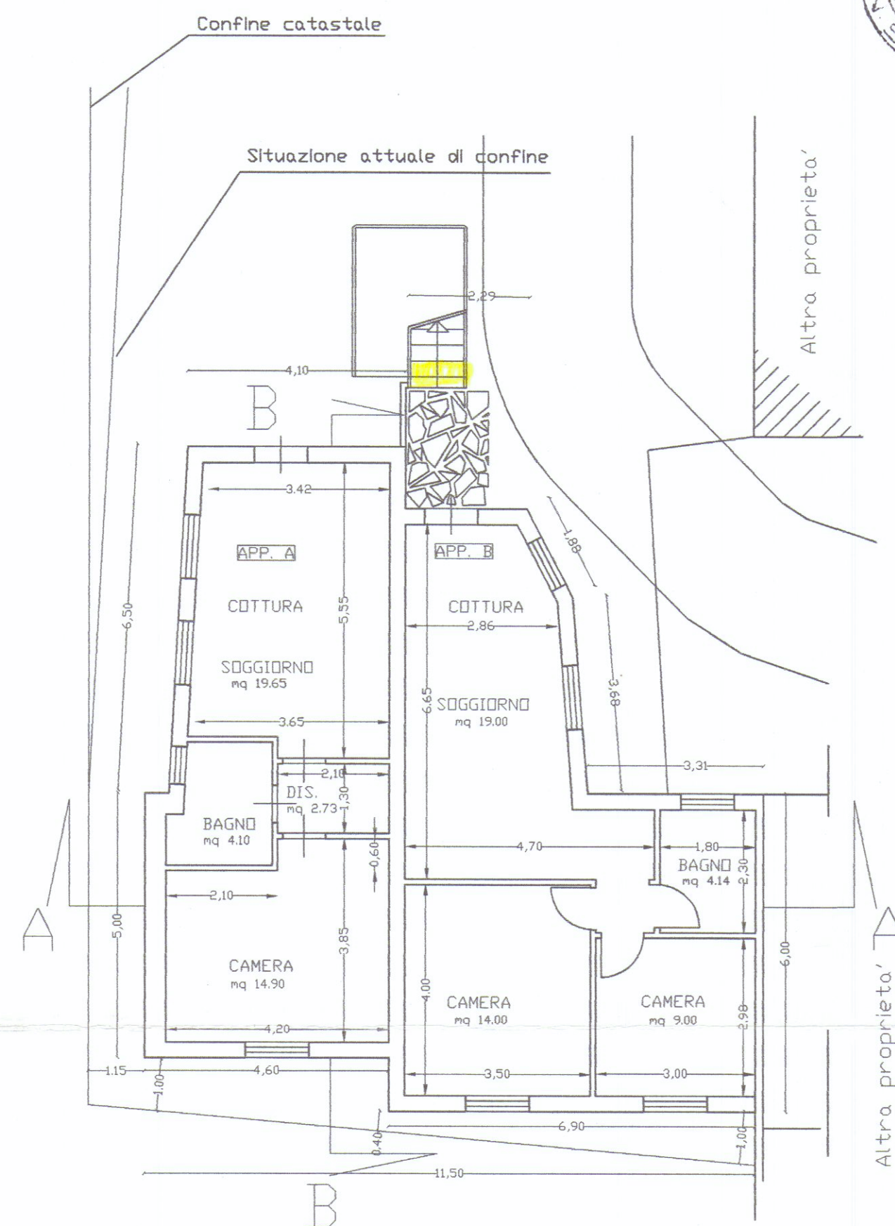
PIANO TERRA
