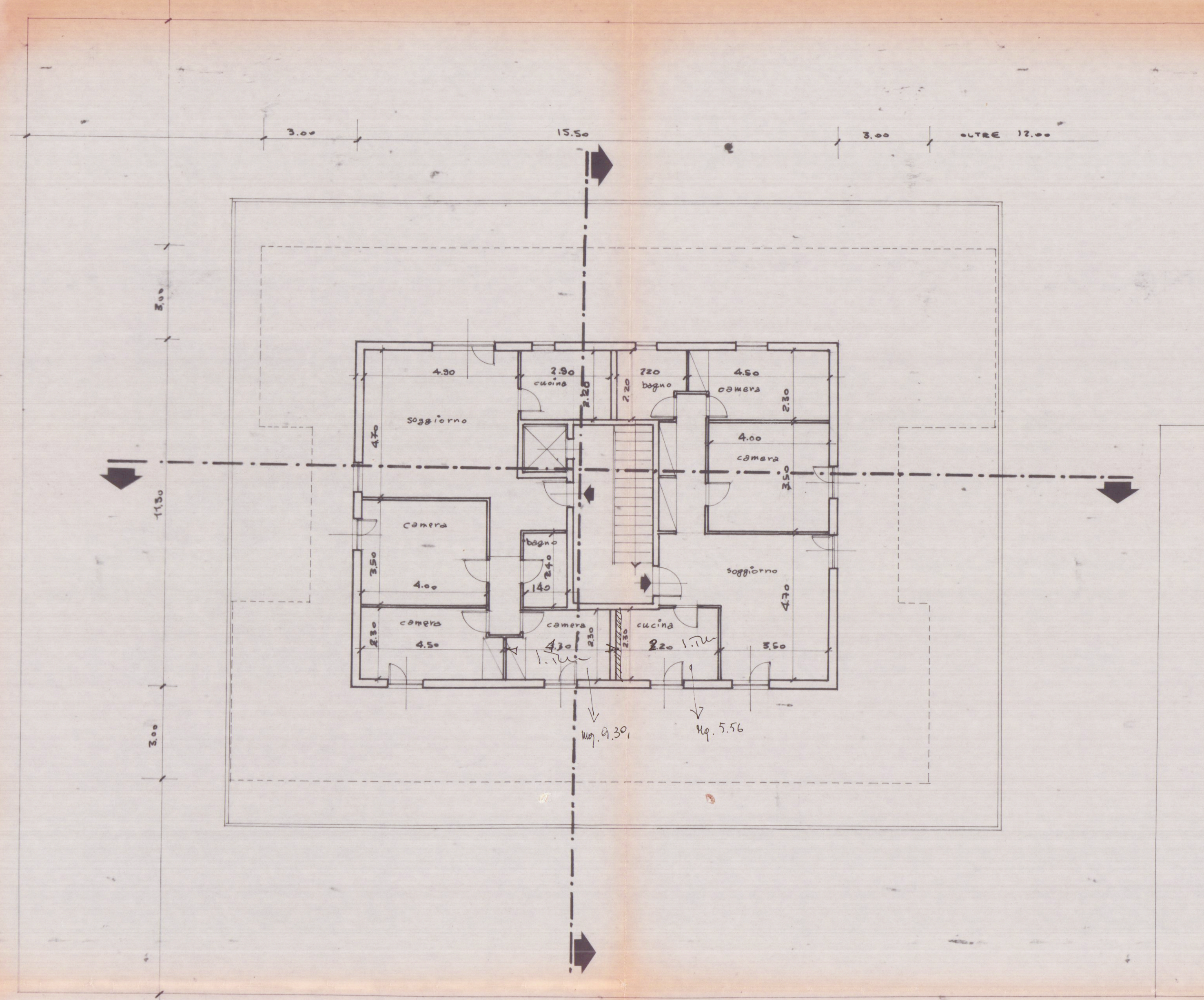
PIANO ATTICO
