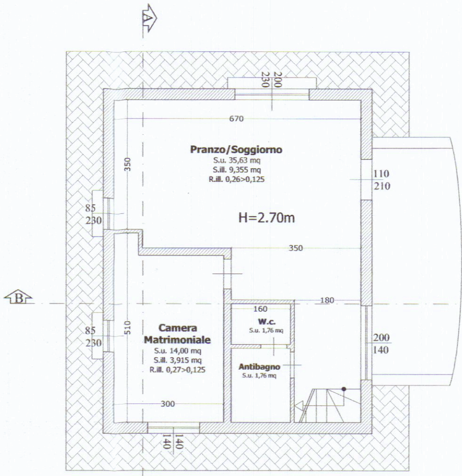
PIANO TERRA
