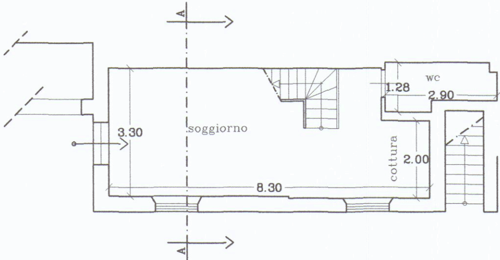
PIANO TERRA
