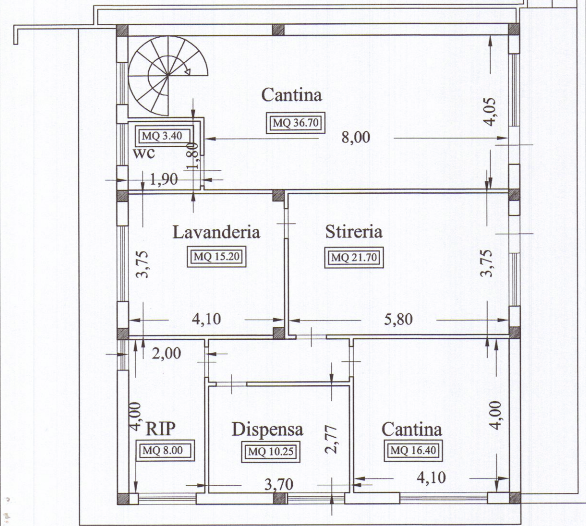
PIANO SEMINTERRATO
