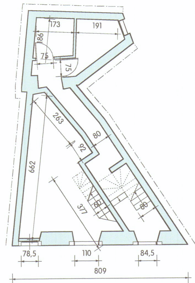
1 piano piano terra scala 1: 100
