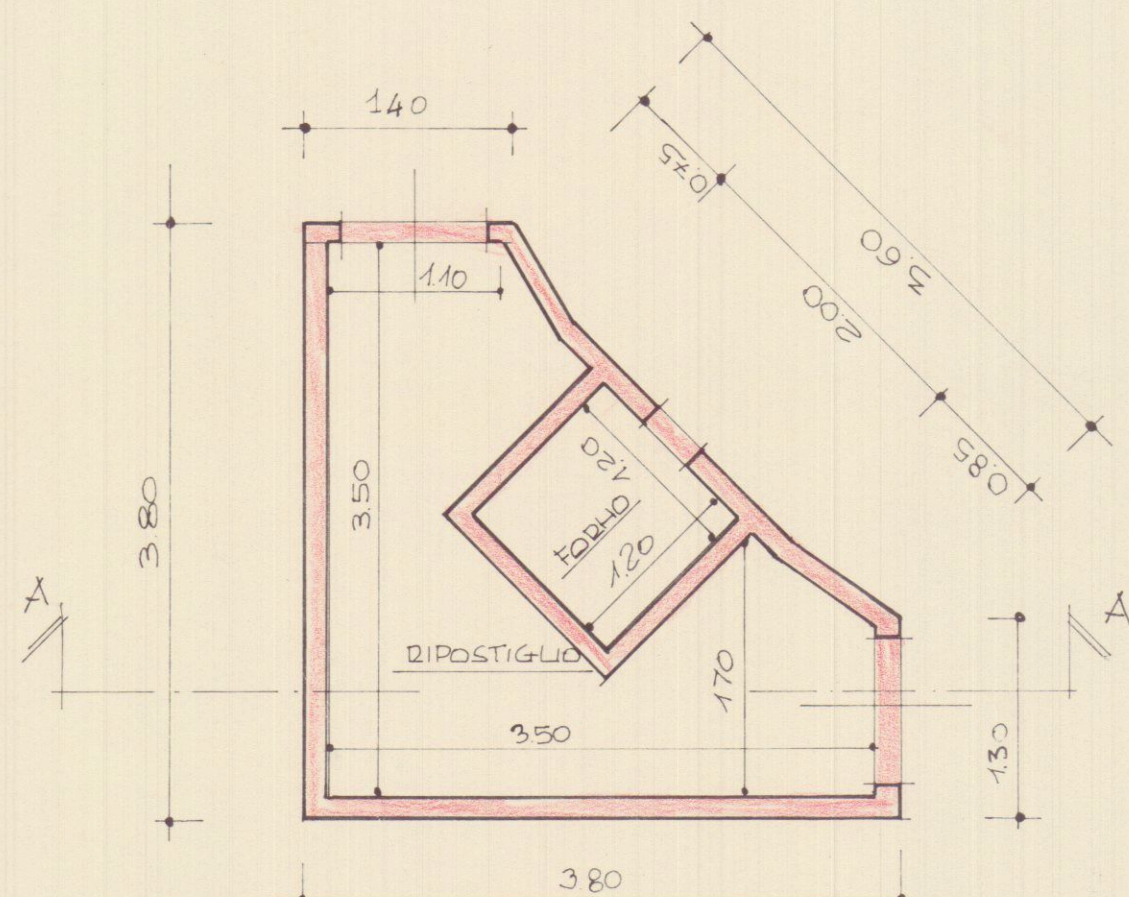
PIANO TERRA
