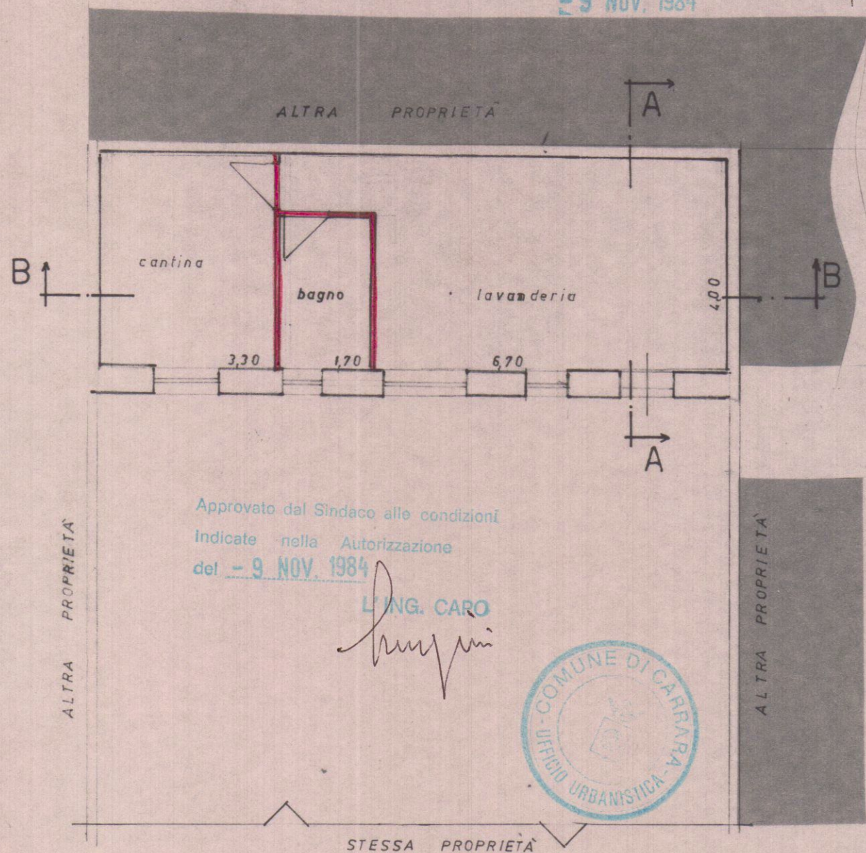
PIANO TERRA
