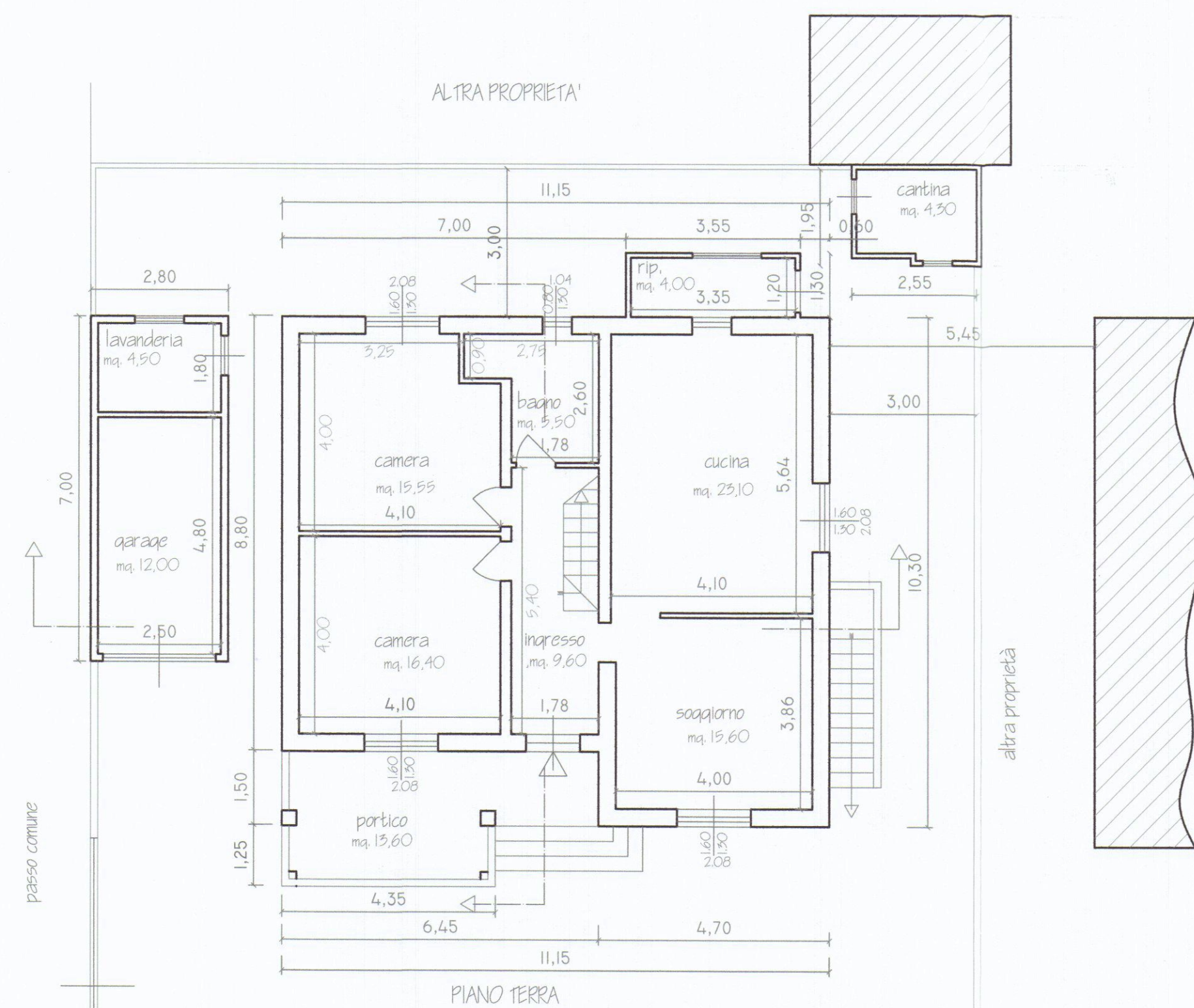
PIANO TERRA
