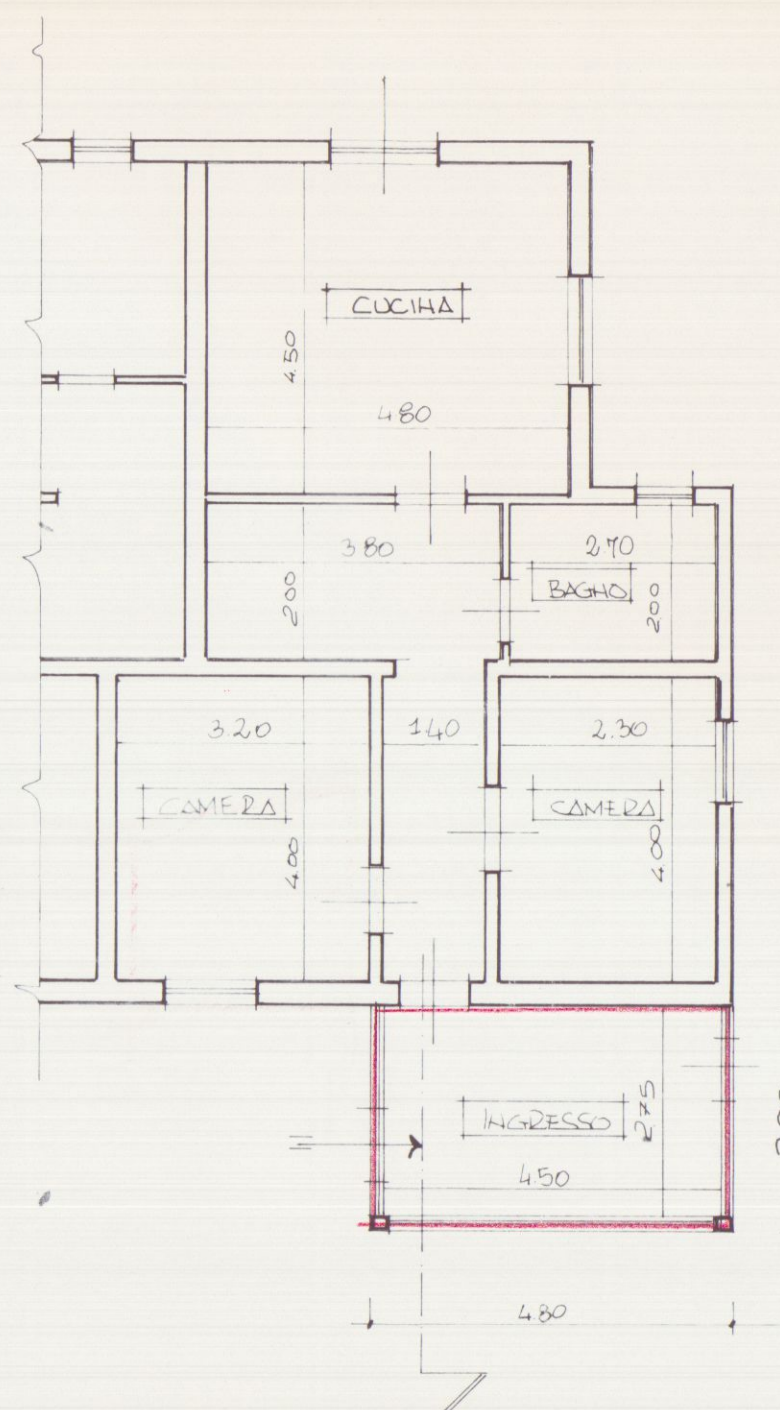
PIANO TERRA
