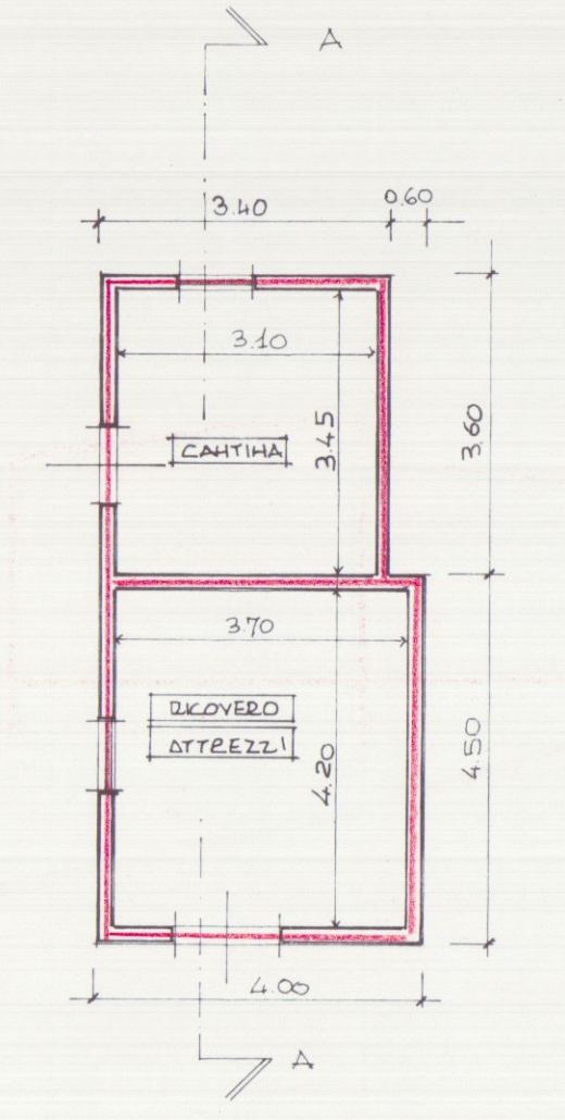
PIANO TERRA
