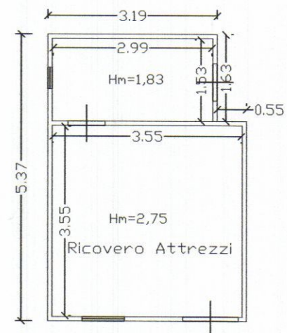
PIANO TERRA
