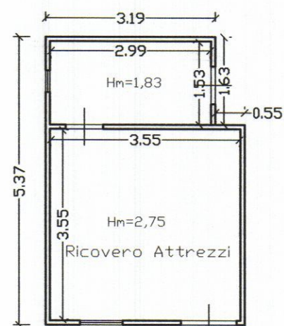
PIANO TERRA
