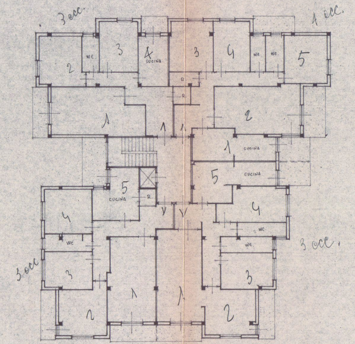
QUARTO PIANO
