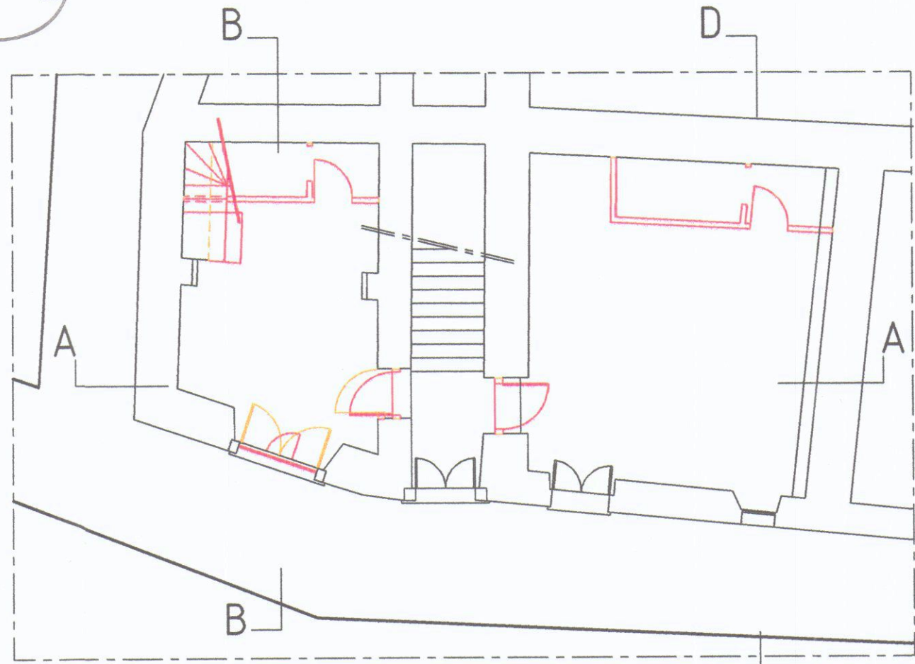
Piano Terra
