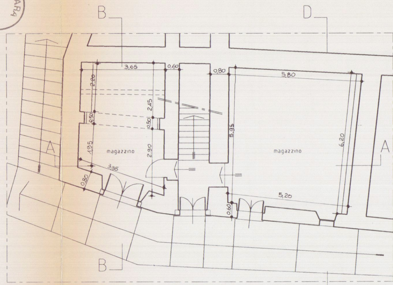
Piano Terra
